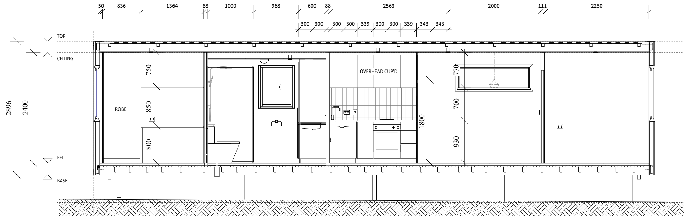
X1 Section 4 100 scale 1:50
