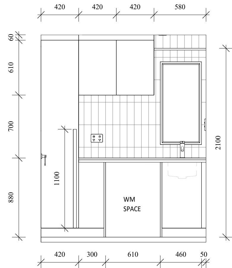
B1 ELEVATION B1 100 scale 1:25
