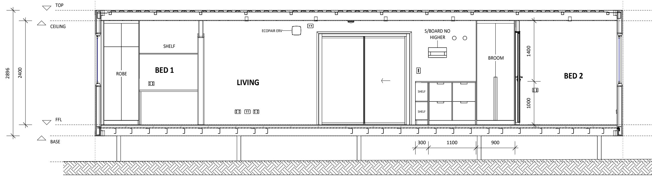
SECTION 1 X2 100 scale 1:50
