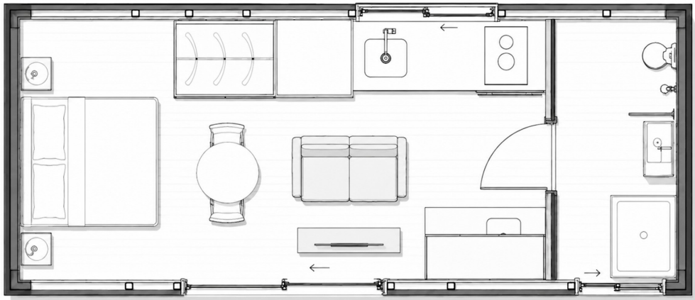
FLOOR PLAN
